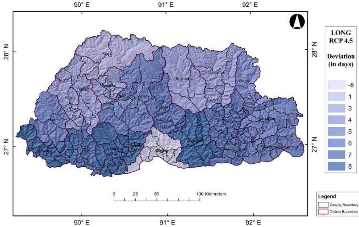
Figure FH 39: Change in number of events with >100 mm in 3 days relative to the baseline {RCP 4.5 - (2070-2099 over 1976-2005)}
