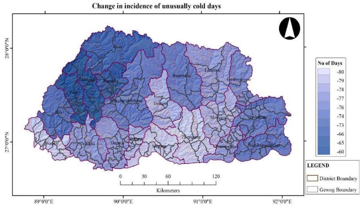
Figure FH 73: Bhutan - Change in incidence of unusually cold days {RCP 8.5 - (2070-2099 over 1976-2005)}
