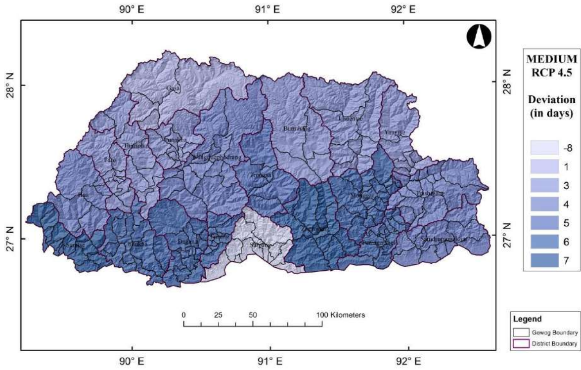
Figure FH 26: Change in number of events with >100 mm in 3 days relative to the baseline {RCP 4.5 - (2051-2069 over 1976-2005)}
