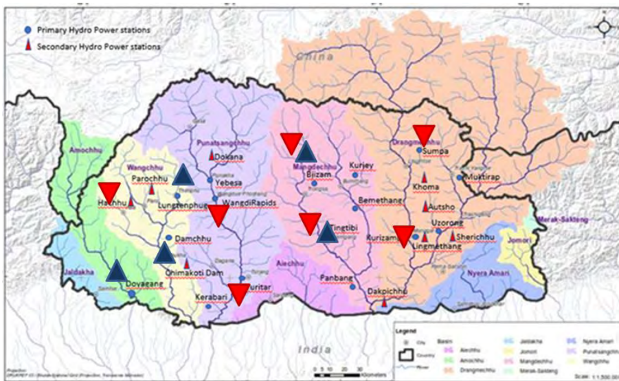
Figure 7.3 Stations with maximum change in low flow periods (red) based on top down analysis: 1. Sumpa / Kurizampa on Kurichu, 2. Tingtibi/Bjizam on MangdeChhu, 3. Toritar/ Wangdue rapids on PunatsangChhu, 4. Sumpa on KhomaChhu, 5. Haa on HaaChhu. Stations with maximum change in peak flow (blue): 1. Damchoe/ Chimakoti on WangChhu, 2. Tingtibi on MangdeChhu, 3. Lungtenphu on Thimphu Chhu, 4. AmoChhu, 5. Bjizam on MangdeChhu.
