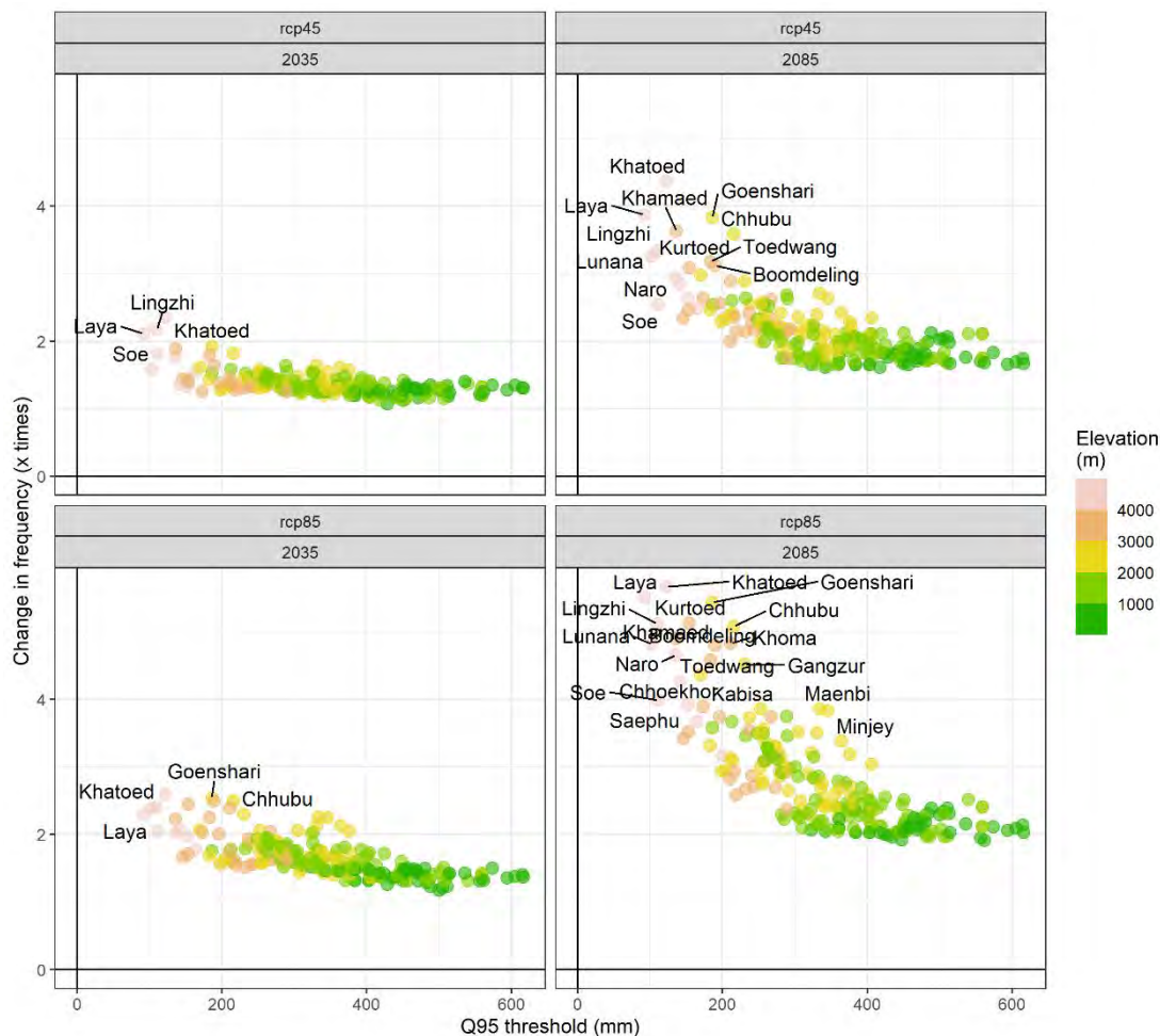
Figure 5.8 . Scatter plot Q95 threshold of 7-day total precipitation (mm) per Gewog and changes in the landslide risk frequency (y-axis) under RCP4.5, 8.5 and 2035 and 2085. The color scale shows the average elevation (m) of each Gewog.
