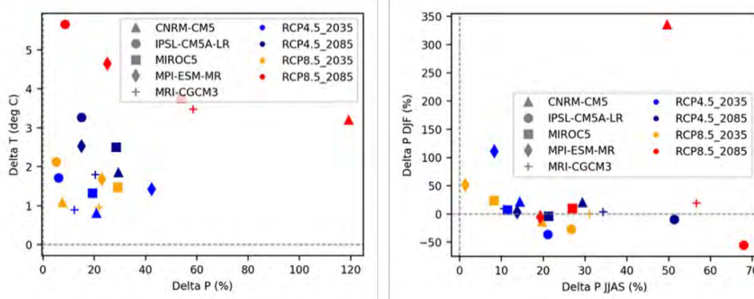
Figure 4.1 Left: Mean annual deltas for temperature T (in ^{\circ}\text{C} ) as a function of mean annual deltas for precipitation P (%) for each of the 20 climate projections (5 GCMS, 2 RCPs, near future 2035 and far future 2085) spatially averaged over Bhutan. Right: Mean annual deltas for precipitation P during the dry winter period of December until February DJF (in %) as a function of mean annual deltas for precipitation P during the wet summer period of June until September JJAS (in %) for each of the 20 climate projections (5 GCMS, 2 RCPs, near future 2035 and far future 2085) spatially averaged over Bhutan.
