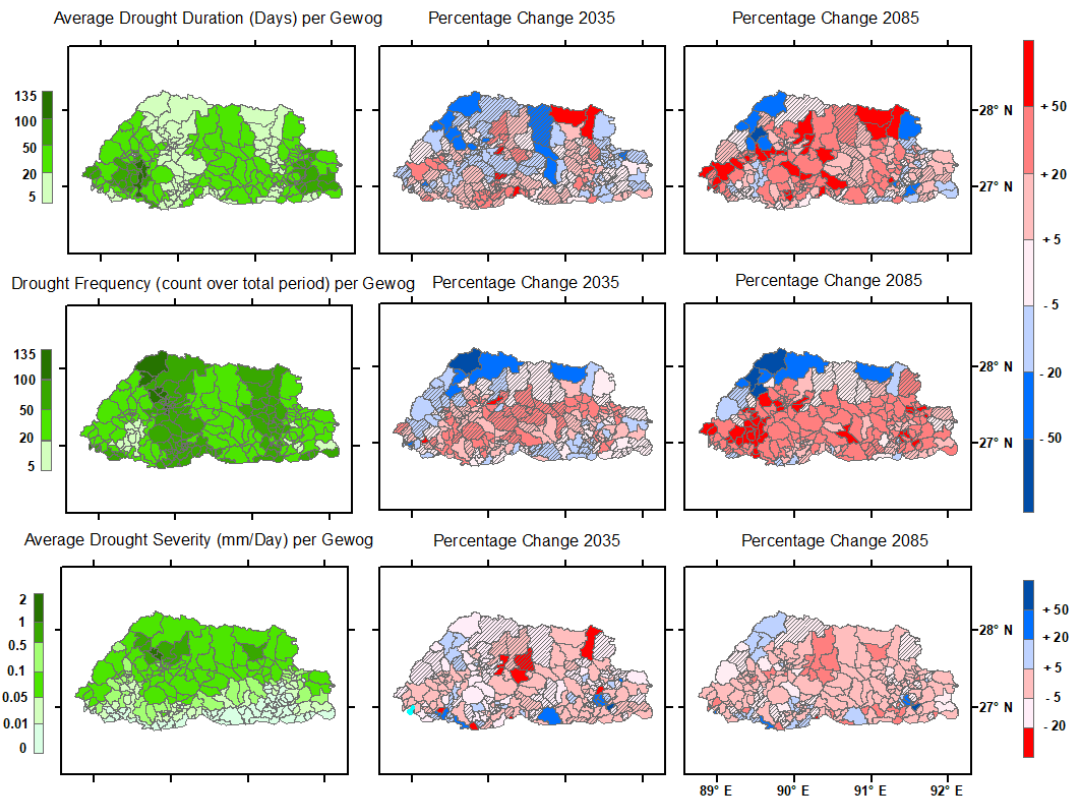
Figure 5.1 Dry spells (defined here as groundwater recharge < 10 percentile) duration, frequency and intensity under historic climate (left column) and future climate (2035 and 2085) for RCP4.5. Hatched areas indicate gewogs where no more than 3 GCMs project the same direction of change. See annex B for RCP8.5.
