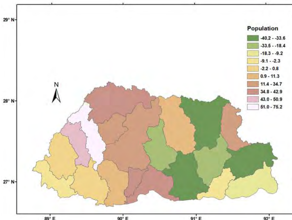
Figure 2.4 Projection of population change in 2042 (%) NSB.
