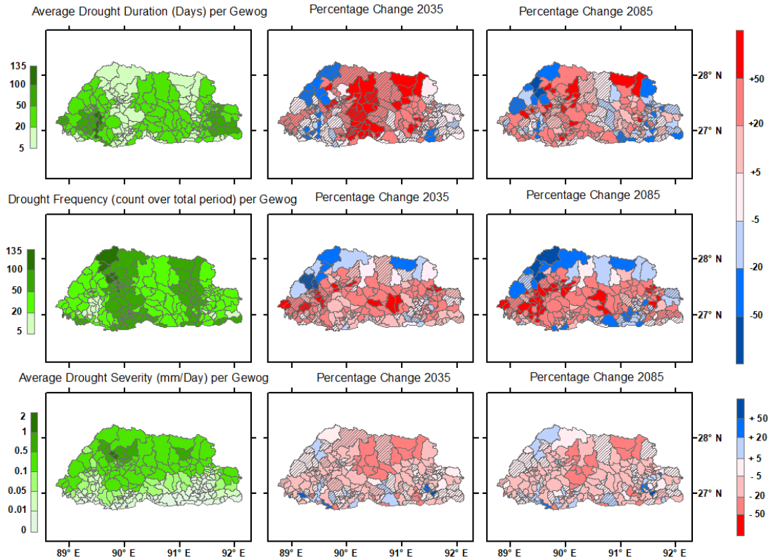
Figure B.1 Dry spells (defined here as groundwater recharge < 10 percentile) duration, frequency and intensity under historic climate (left column) and future climate (2035 and 2085) for RCP8.5. Hatched areas indicate gewogs where no more than 3 GCMs project the same direction of change.
