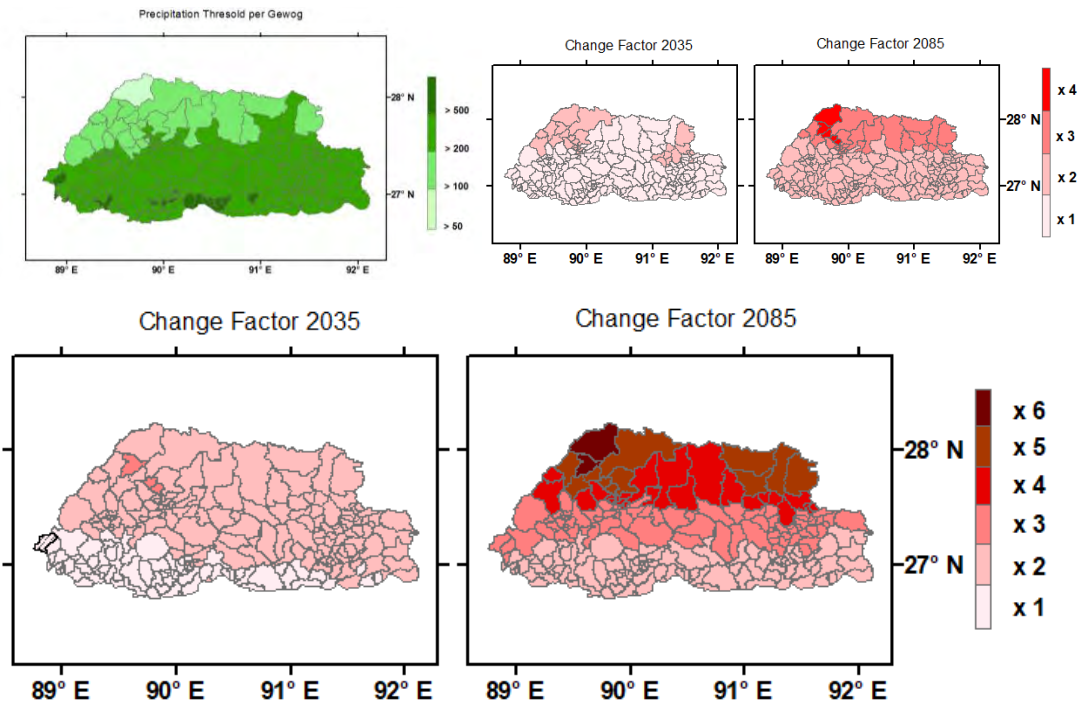
Figure 5.7. Changes in the 7-day accumulated precipitation occurrences above the Q95 threshold at the Gewog level. The upper left map shows in mm the Q95 values per gewog. The other maps show the ratio of changes from the historical frequencies for the years 2035 and 2085 respectively for RCP4.5 (upper) and RCP8.5 (lower). Hatched areas indicate gewogs where no more than 3 GCMs project the same direction of change.
